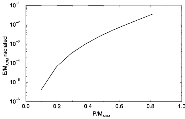
FIG. 1. The energy radiated in the “relaxation” of a single, boosted Bowen-York black hole to a Schwarzschild black hole, as a function of the momentum. At about P/M_{ADM} \sim 0.4 the radiation is equivalent to the total energy radiated in a “close limit” collision of two boosted black holes.
