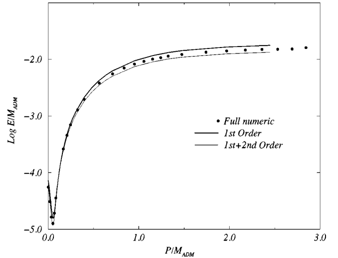
FIG. 2. The energy radiated in the head-on collision of two boosted black holes as calculated in Ref. [10]. The collision is for two black holes separated by a Misner parameter \mu_0 = 1.5 . Depicted are the results of first and second order perturbation theory and the full numerical results of the NCSA-Potsdam-WashU group. We see that the collisions never radiate more than 1% of the ADM mass in gravitational waves.
